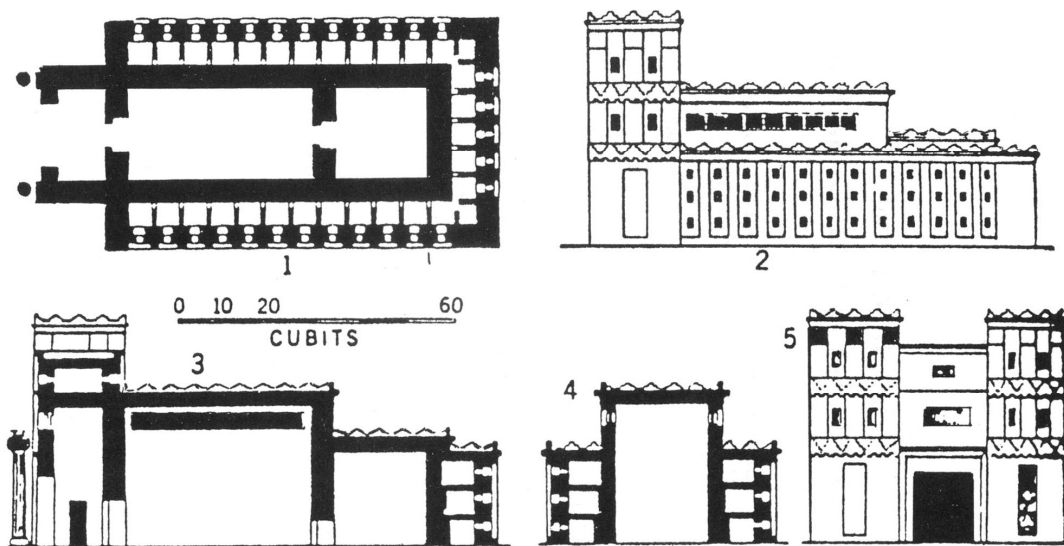
(1) Ground plan; (2) Side view; (3) Longitudinal cross-section; (4) Breadth cross-section; (5) front view. From Vincent-Steve, Jerusalem de l'Ancien Testament , J. Gabalda & Cie., Paris 1956, tome 11.
